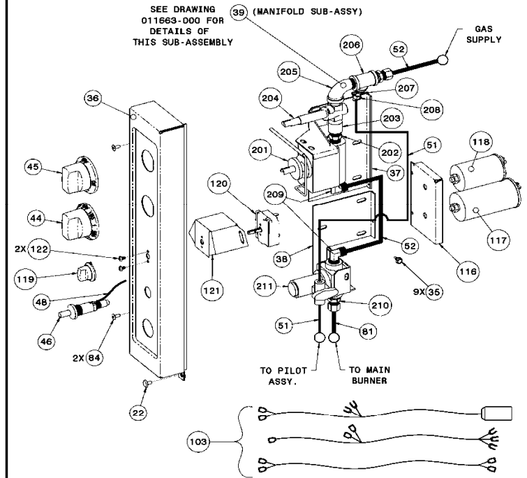
CONTROLS ASSY.
