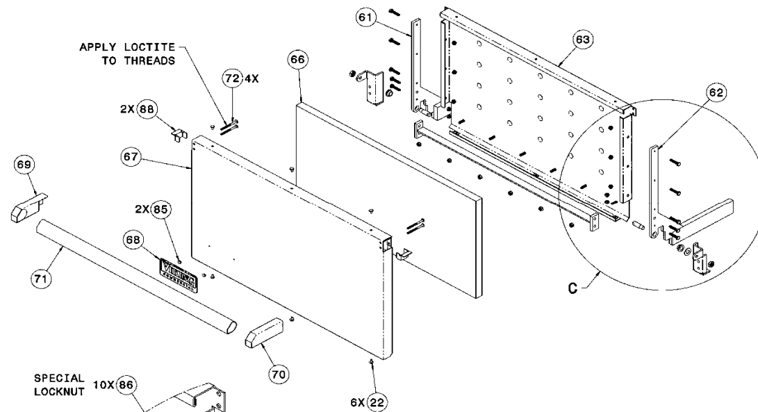
DOOR ASSY.
