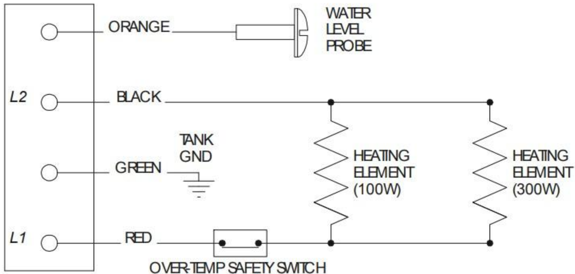
SCHEMATIC FOR 240V 400W 5 GAL TANK
