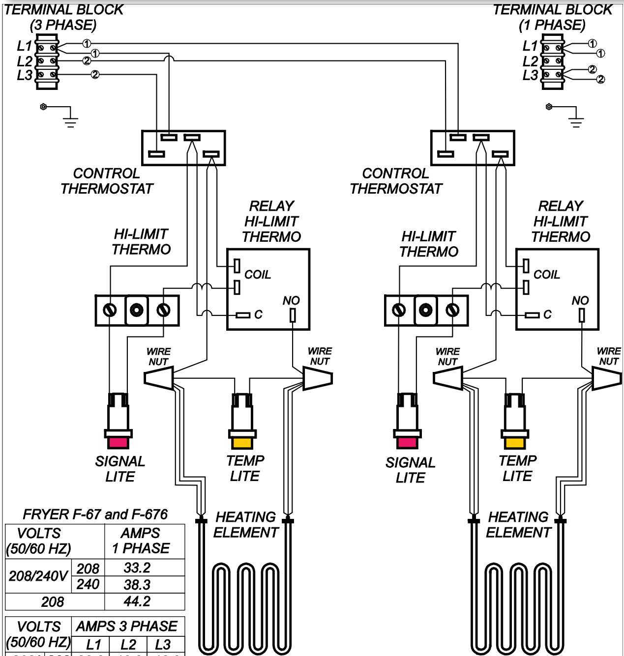
WIRING DIAGRAM F-67 and F-676 p/n 307302
