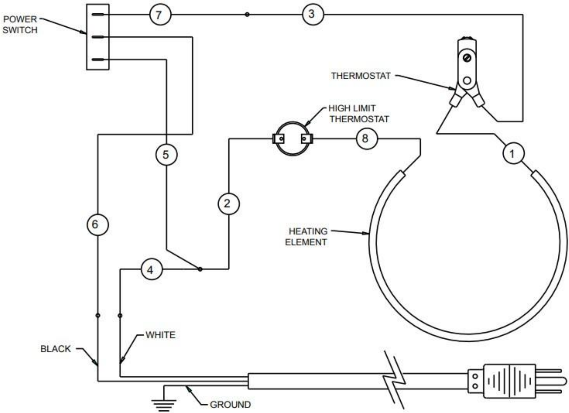
HDW-2 Wiring Diagram
