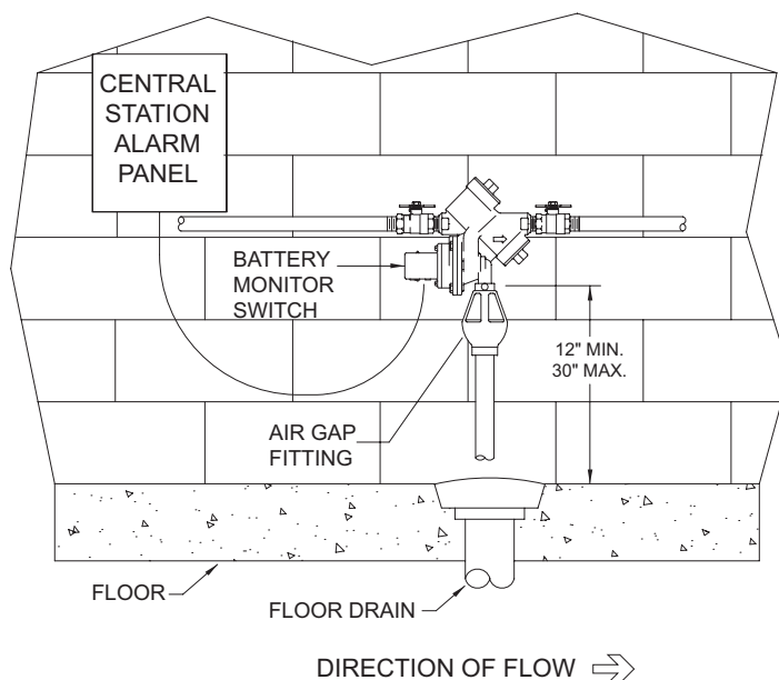
CENTRAL STATION ALARM SYSTEM (INDOOR)
